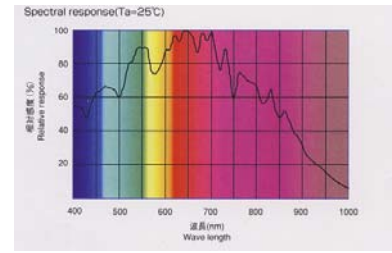
Figure 1: Spectral sensitivity of line CMOS camera
