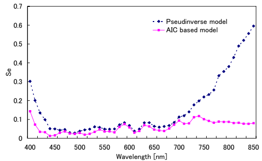
Figure 8: Residual sum of squares in wavelength region.
