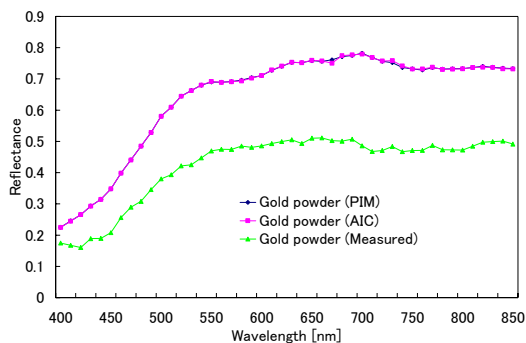
Figure 9: Spectral reflectance reconstruction of glossy target
