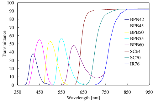
Figure 6: Transmittance of selected filter
