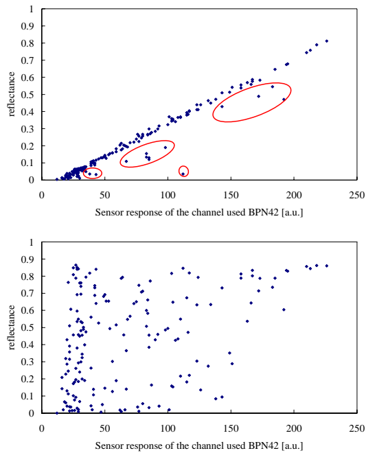
Figure 4: Scatter chart of sensor response of the channel which used BPN42 filter and reflectance (a) Reflectance at 440 nm. The data points that deviated from linear correlation are circled. (b) Reflectance at 700 nm.
