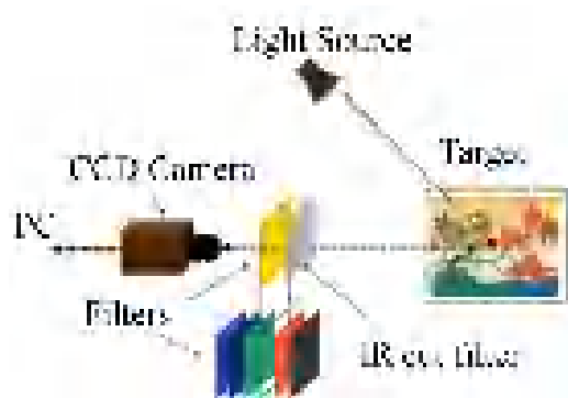
Figure 1: Schematic representation of the multispectral imaging set-up
